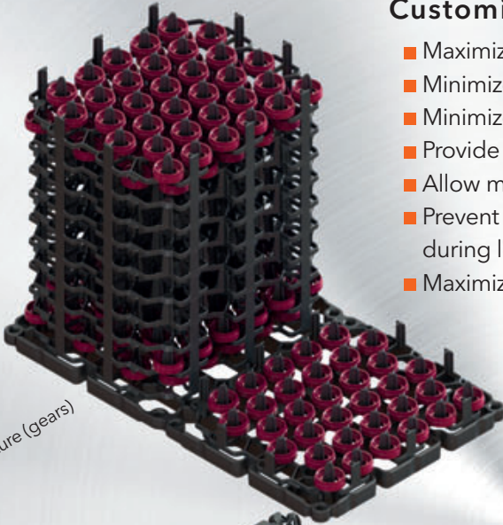
LPC fixture (ring gears)
